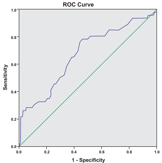
Figure 3. ROC curve for BA.
